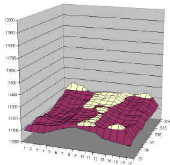
Figure 4 - surface contour map of a store with bad frostheave - here the worst areas have lifted by 200mm
