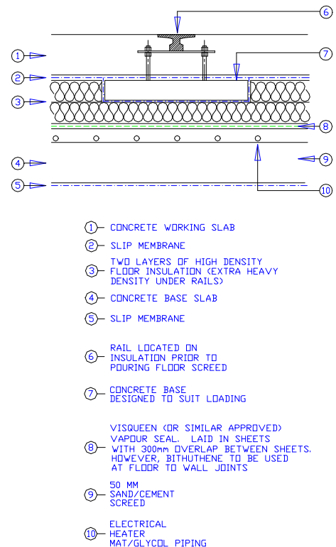
Figure 1 - General Sub-Zero Floor Construction
